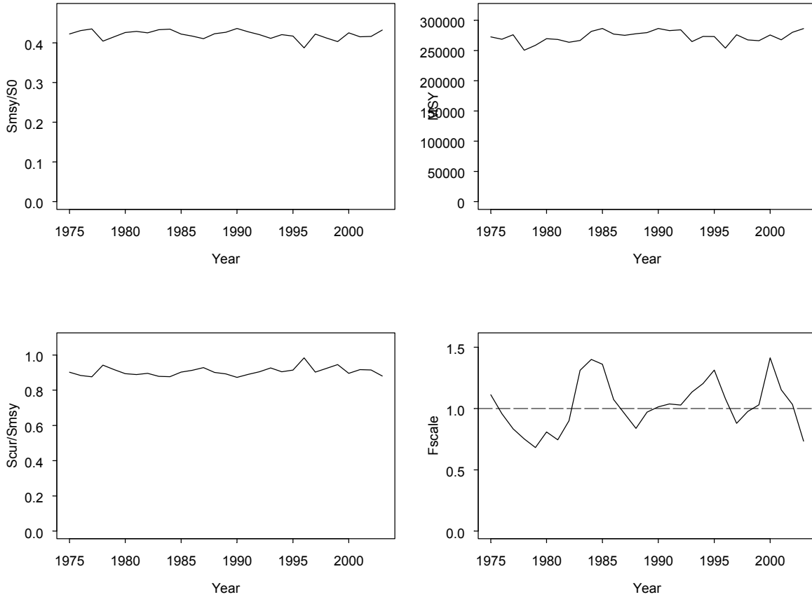
FIGURE 4.12c. Estimates of AMSY-related quantities calculated using the average age-specific fishing mortality for each year. ( S_{cur} is the spawning biomass at the start of 2005). See the text for definitions.
