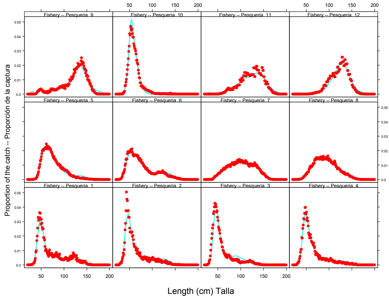
FIGURE 4.2. Average observed (dots) and predicted (curves) size compositions of the catches taken by the fisheries defined for the stock assessment of yellowfin tuna in the EPO.
