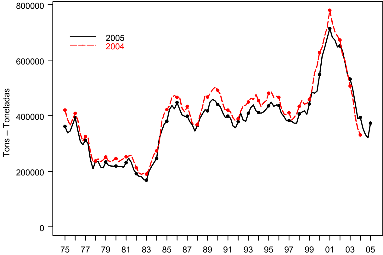
FIGURE 4.12a. Comparison of estimated biomasses of yellowfin tuna in the EPO from previous assessments and the current assessment. t = metric tons.
