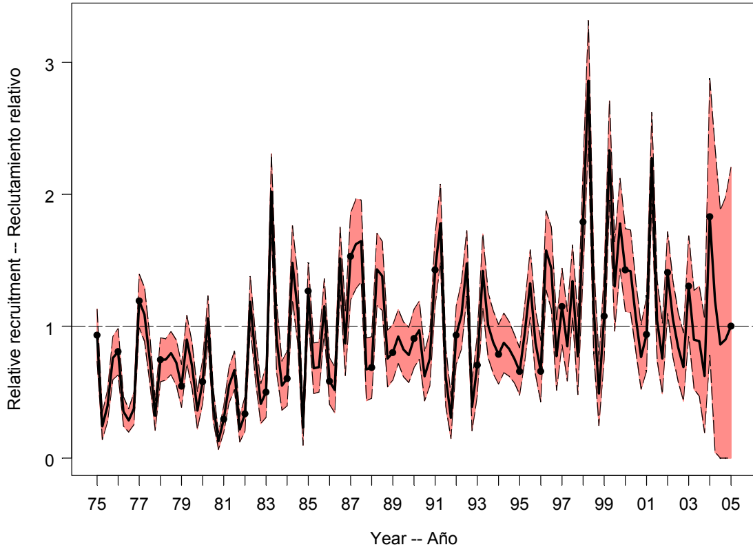
FIGURE 4.7. Estimated recruitment of yellowfin tuna to the fisheries of the EPO. The estimates are scaled so that the average recruitment is equal to 1.0. The bold line illustrates the maximum likelihood estimates of recruitment, and the shaded area indicates the approximate 95% confidence intervals around those estimates. The labels on the time axis are drawn at the start of each year, but, since the assessment model represents time on a quarterly basis, there are four estimates of recruitment for each year.
