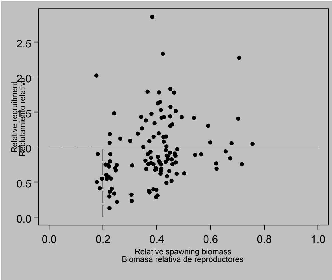
FIGURE 4.6. Estimated relationship between recruitment of yellowfin tuna and spawning biomass. The recruitment is scaled so that the average recruitment is equal to 1.0. The spawning biomass is scaled so that the average unexploited spawning biomass is equal to 1.0.
