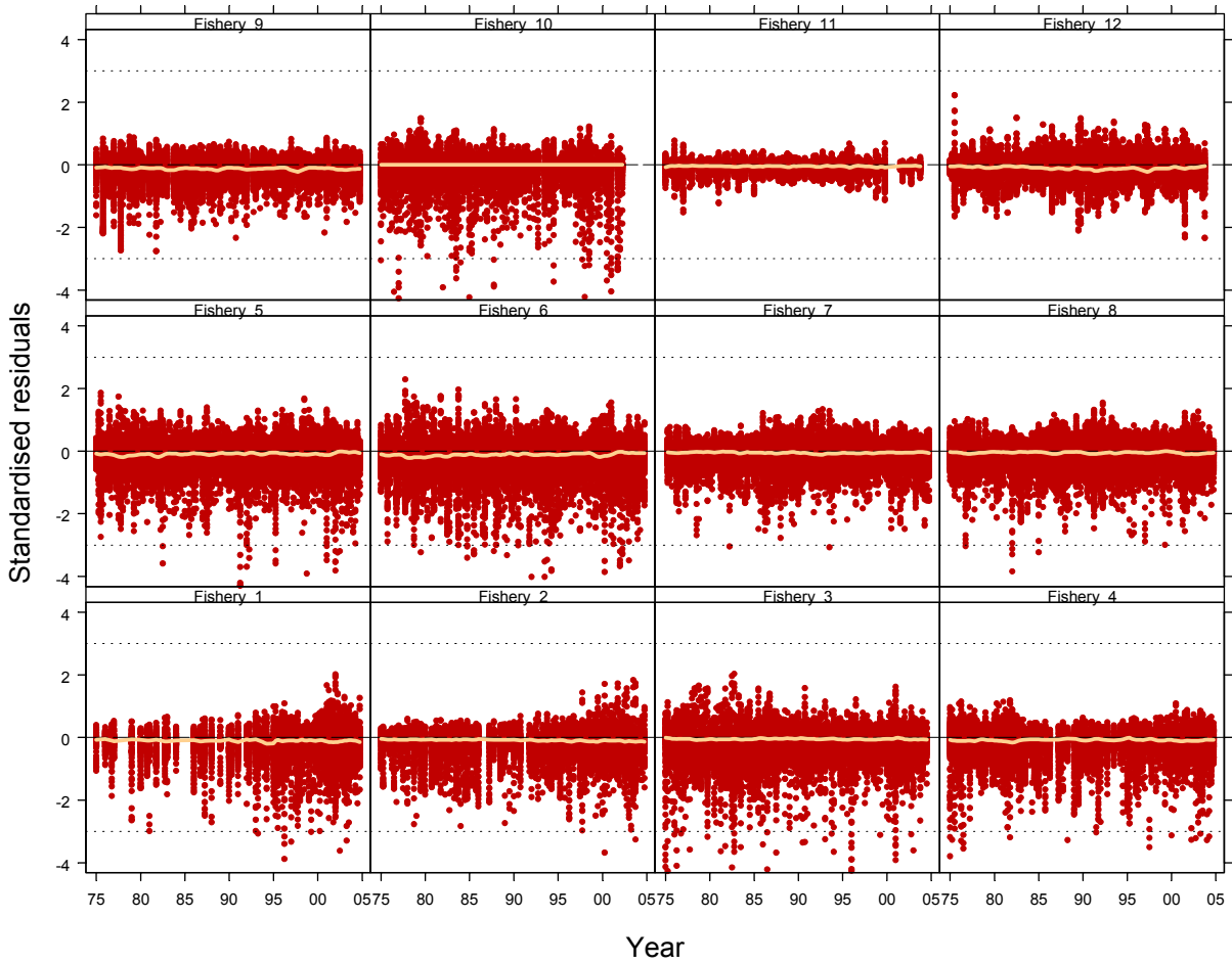
FIGURE C.2. Standardized residuals for the length-frequency data of yellowfin tuna by time. The dotted horizontal lines represent three standard deviations on either side of the mean.
