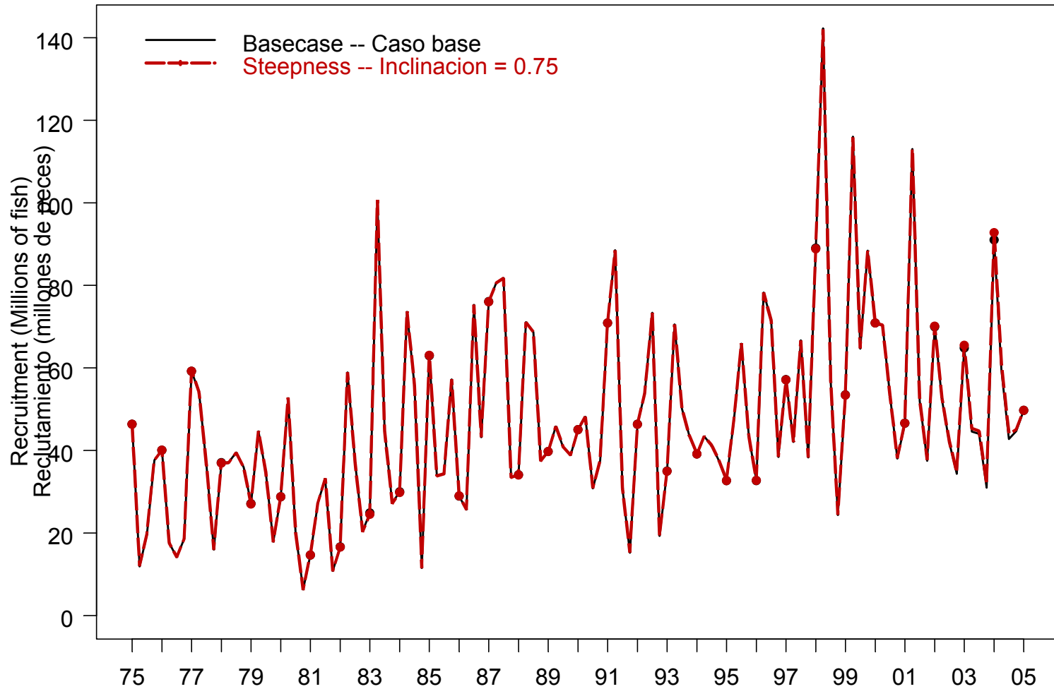
FIGURE A.2. Comparison of estimates of recruitment of yellowfin tuna from the analysis without a stock-recruitment relationship (base case) and with a stock-recruitment relationship (steepness = 0.75).
