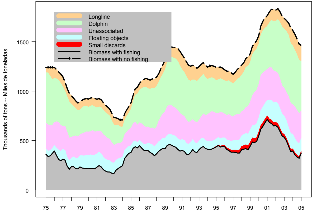
FIGURE 4.10c. Biomass trajectory of a simulated population of yellowfin tuna that was not exploited during 1975-2004 (dashed line) and that predicted by the stock assessment model (solid line). The shaded areas between the two lines show the portions of the fishery impact attributed to each fishing method. t = metric tons.
