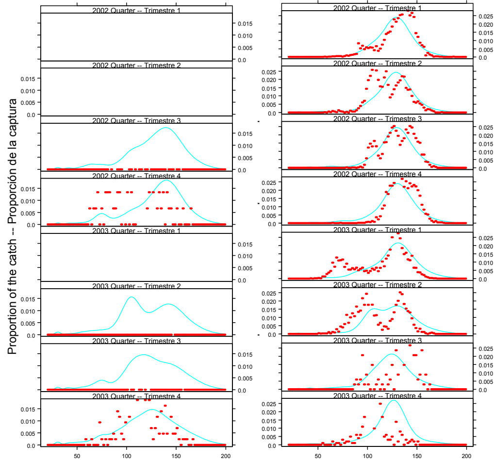
FIGURE 4.8e. Observed (dots) and predicted (curves) size compositions of the recent catches of yellowfin tuna by the longline fishery (Fishery 12).
