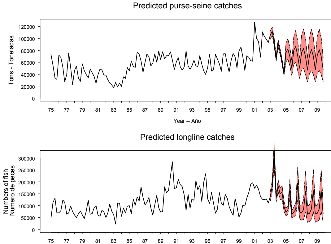
FIGURE 6.3. Catches of yellowfin tuna during 1975-2004 and simulated catches of yellowfin tuna during 2005-2009 by the purse-seine and pole-and-line fleets (upper panel) and the the longline fleet (lower panel), using the likelihood profile method. The thin dashed lines represent the estimated 95% confidence limits of the estimates. The estimates after 2005 indicate the catches predicted to occur if the effort continues at the average of that observed in 2004, catchability (with effort deviates) continues at the average of that observed in 2002 and 2003, and average environmental conditions occur during the next 5 years. t = metric tons.
