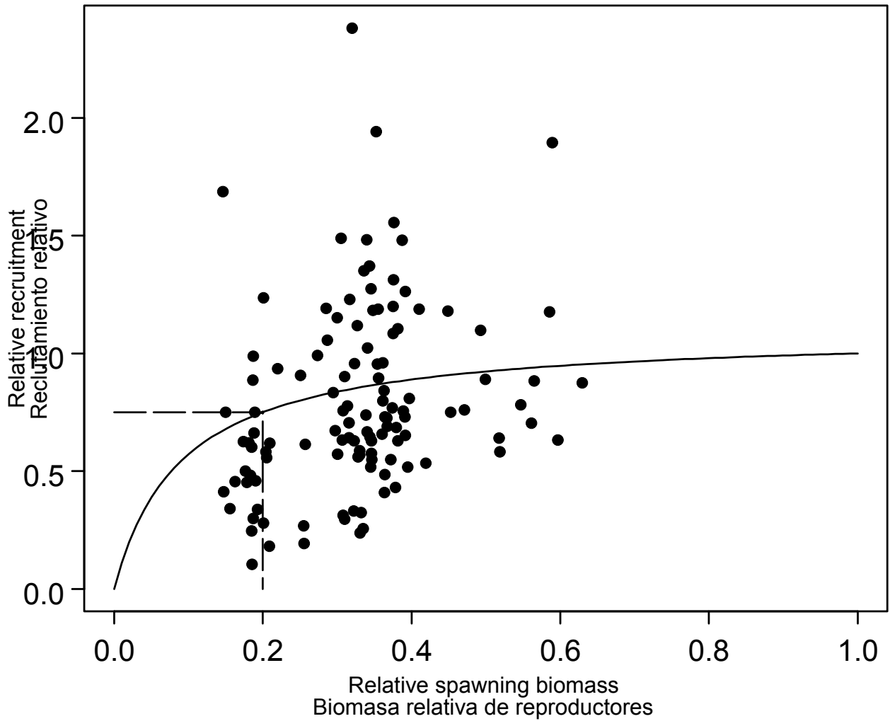
FIGURE A.5. Recruitment plotted against spawning biomass of yellowfin tuna when the analysis has a stock-recruitment relationship (steepness = 0.75).
