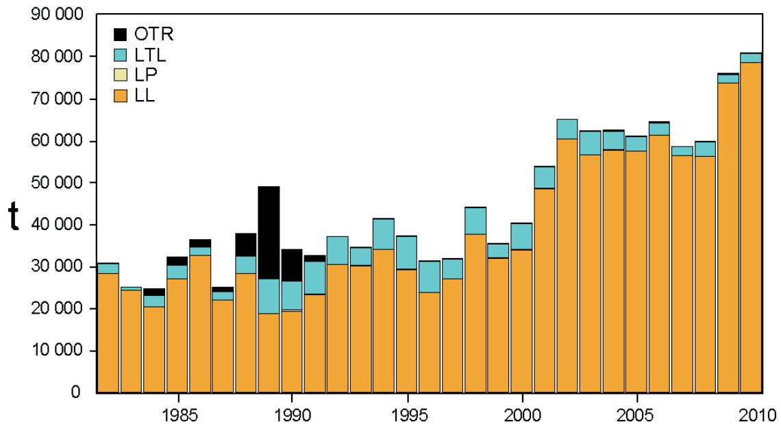
FIGURE F-1b. Retained catches of South Pacific albacore. FIGURA F-1b. Capturas retenidas de albacora del Pacífico sur.
