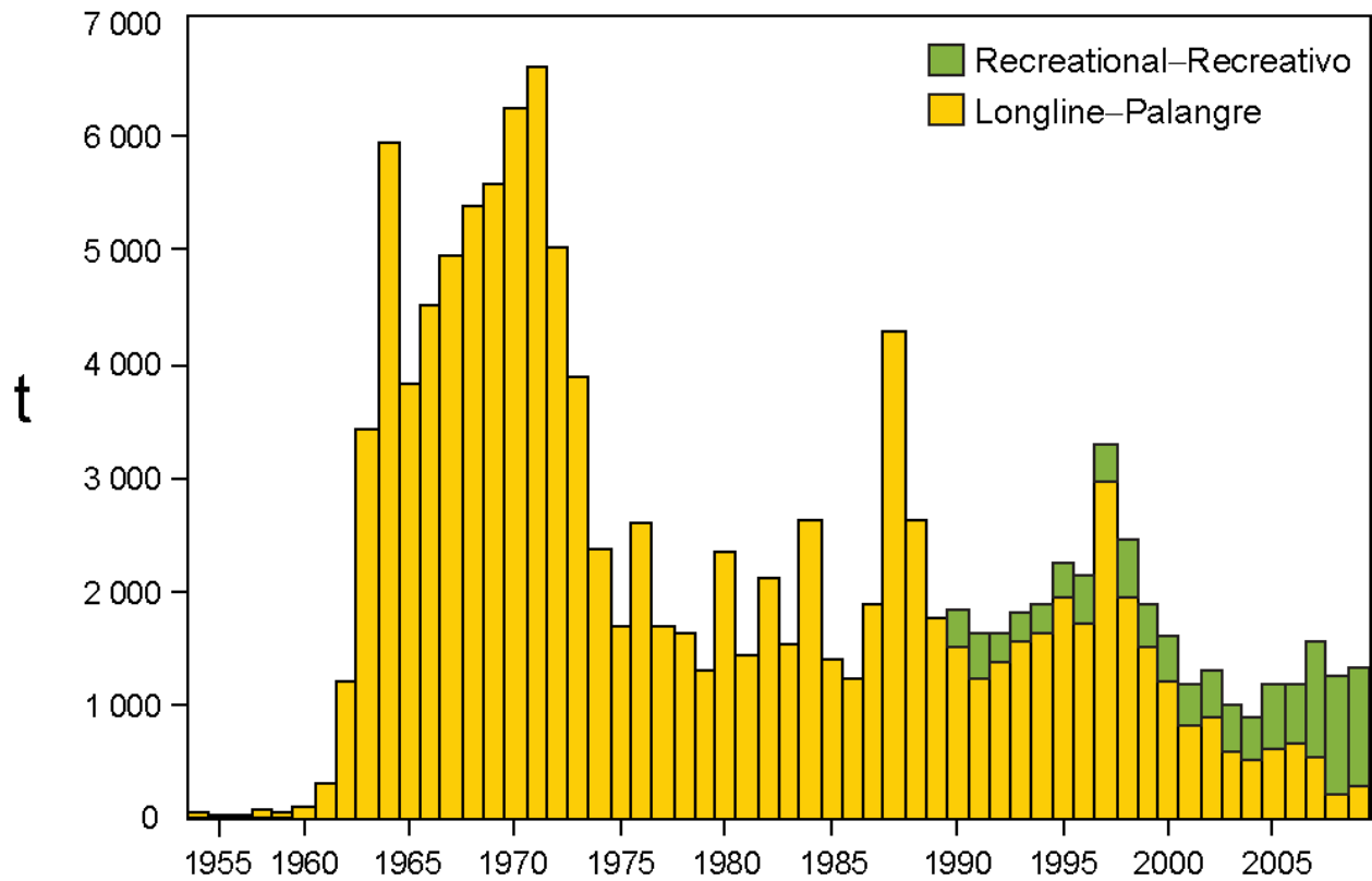
FIGURE I-1. Landings of striped marlin from the northern EPO by longline and recreational fisheries, 1954-2009. FIGURA I-1. Descargas de marlín rayado del OPO norte por las pesquerías palangreras y recreativas, 1954-2009.
