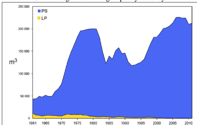
Figure 2. Carrying capacity, in cubic meters of well volume, of the purse-seine and pole-and-line fleets in the EPO, 1961-2011
