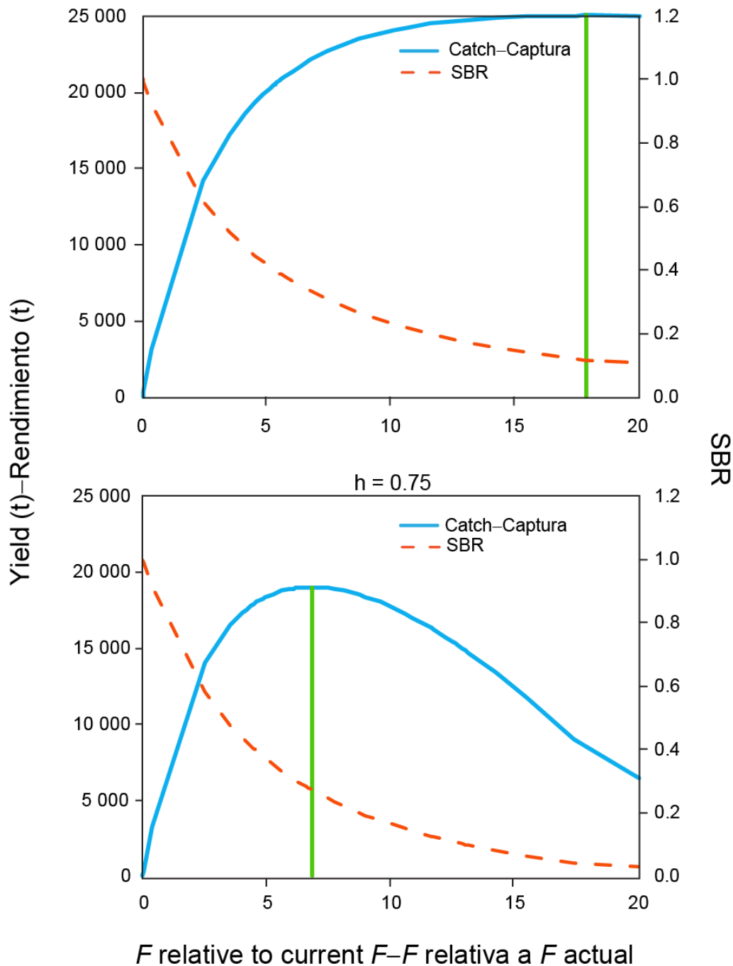
FIGURE 4.2.2.2. Estimated yield and spawning biomass ratio (SBR), from the assessment (upper panel) and from the model with a steepness ( h ) of 0.75 (lower panel), as a function of fishing mortality relative to the current level of fishing mortality. The green vertical bar indicates the relative fishing mortality expected to provide catch at the level of maximum sustainable yield (MSY).
