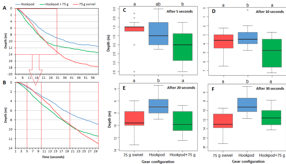
Figure 3. Average sinking profiles of baited hooks with 75 g leaded swivels (red), Hookpod only (blue) or Hookpod plus 75 g leaded swivel (green, A), and detail of the first 30 seconds after deployment, with the 5, 10, 20 and 30 seconds thresholds highlighted with red vertical lines (B). The boxplots show the depth distribution (median and the 25th and 75th percentiles, whiskers indicate values within 1.5 times of the interquartile range, and black circles indicate outliers) of baited hooks of each gear treatment after 5 (C), 10 (D), 20 (E) and 30 (F) seconds of deployment. Boxplots not sharing the same lower-case letters denote statistically distinct treatments ( P < 0.05 , Tukey test).
