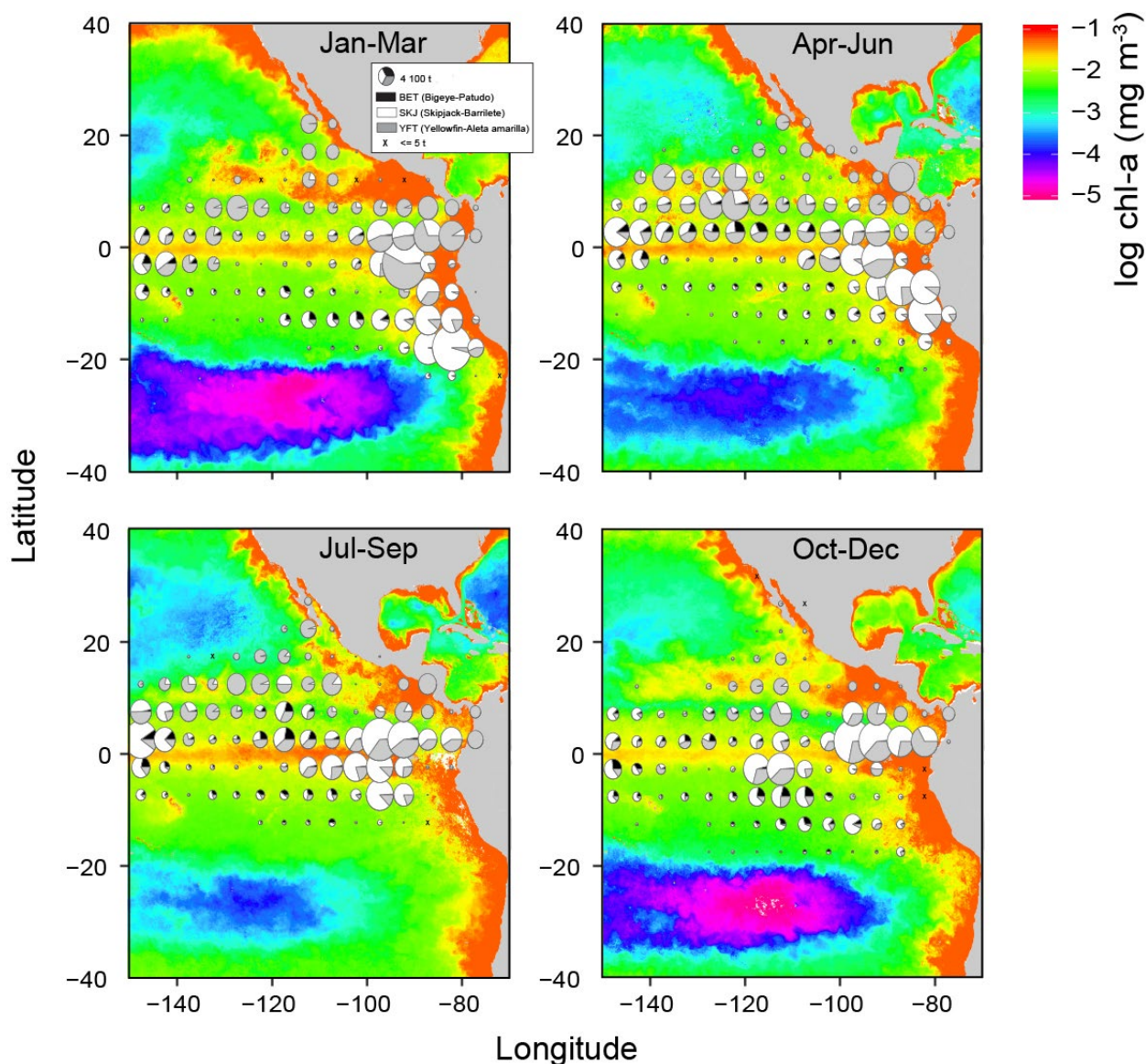
FIGURE L-11. Mean log chlorophyll-a concentration (in \text{mg m}^3 ) for each quarter during 2022 with catches of tropical tunas overlaid. Chlorophyll data obtained from NOAA CoastWatch on March 3, 2023, “Chlorophyll-a, Aqua MODIS, NPP, L3SMI, Global, 4km, R2022 SQ, 2003-present (Monthly Composite)”, NOAA NMFS SWFSC ERD, https://coastwatch.pfeg.noaa.gov/erddap/info/erdMH1chlamday_R2022SQ/index.html .
