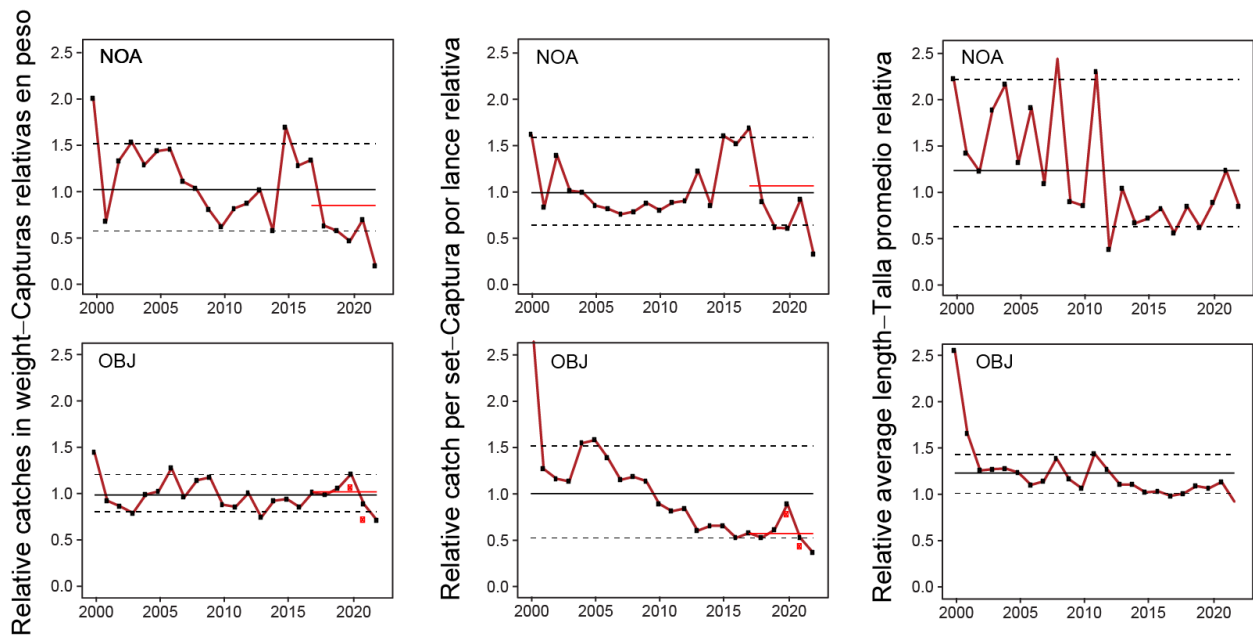
FIGURE D-2. Indicators of catch, catch per set, and average length for bigeye tuna in the EPO based on purse-seine data for 2000-2022. The dashed horizontal lines are the 10 th and 90 th percentiles, and the solid horizontal line is the median. The red dots are the bias-adjusted estimates for floating-object catches in the two COVID-19 years (see SAC-13-05 ). The red dashed lines mark the status quo reference levels (average conditions in 2017-2019).
