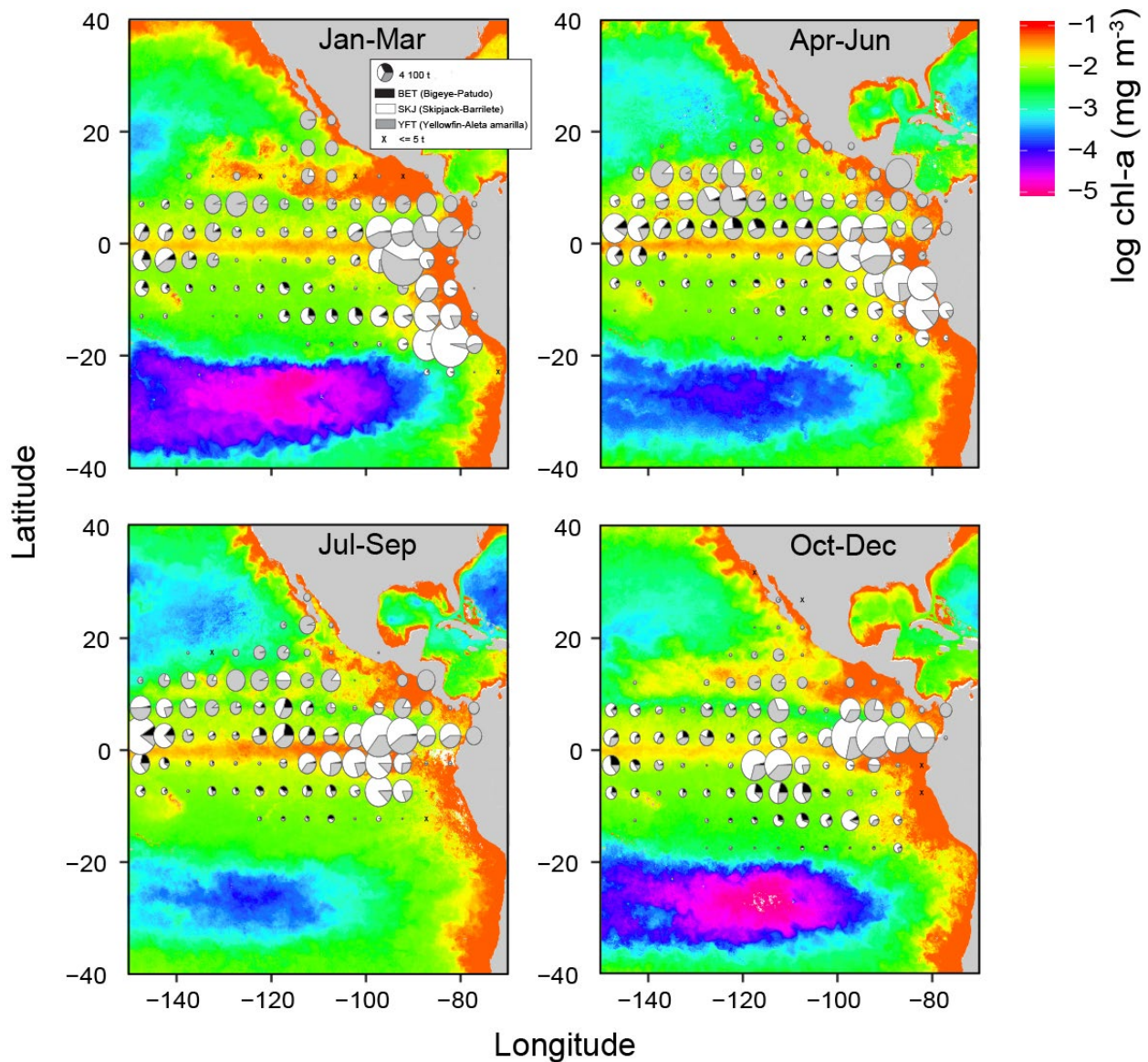
FIGURE L-11. Mean log chlorophyll-a concentration (in \text{mg m}^3 ) for each quarter during 2022 with catches of tropical tunas overlaid. Chlorophyll data obtained from NOAA CoastWatch on March 3, 2023, “Chlorophyll-a, Aqua MODIS, NPP, L3SMI, Global, 4km, R2022 SQ, 2003-present (Monthly Composite)”, NOAA NMFS SWFSC ERD, https://coastwatch.pfeg.noaa.gov/erddap/info/erdMH1chlamday_R2022SQ/index.html .
