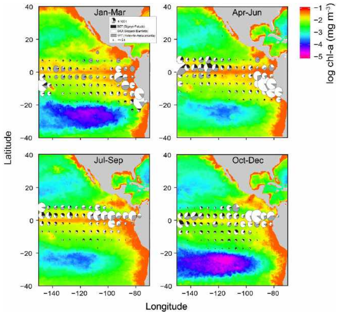
FIGURE L-11. Mean log chlorophyll-a concentration (in \text{mg m}^{-3} ) for each quarter during 2019 with catches of tropical tunas overlaid. Chlorophyll data obtained from NOAA CoastWatch on February 19, 2020, “Chlorophyll, NOAA, VIIRS, Science Quality, Global, Level 3, 2012-present, Monthly”, NOAA NMFS SWFSC ERD, https://coastwatch.pfeg.noaa.gov/erddap/info/nedisVHNSQchlaMonthly/index.html .
