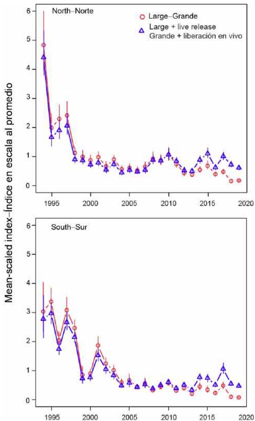
FIGURE K-1. Mean-scaled standardized silky shark bycatch-per-set (BPS; in numbers of sharks per set) in sets on floating objects for large sharks, with and without live release, in the north (top) and south (bottom) EPO. Vertical bars indicate pointwise approximate 95% confidence intervals.
