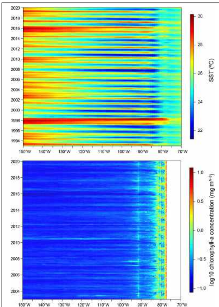
FIGURE L-9. Time-longitude Hovmöller diagram with data averaged across the tropical eastern Pacific Ocean from 5°N to 5°S for mean monthly SST for January 1993–January 2020 (top panel) ( https://www.esrl.noaa.gov/psd/ ) and mean monthly chlorophyll-a concentration for January 2003–January 2020 (bottom panel) ( https://coastwatch.pfeg.noaa.gov/erddap/info/erdMH1chlamday/index.html )
