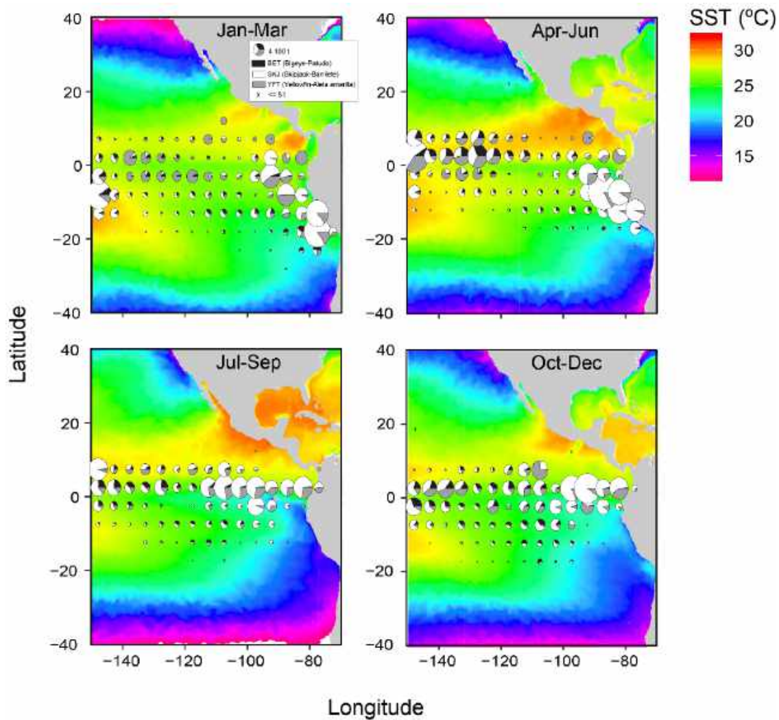
FIGURE L-10. Mean sea surface temperature (SST) for each quarter during 2019 with catches of tropical tunas overlaid. SST data obtained from NOAA NMFS SWFSC ERD on March 5, 2020, “Multi-scale Ultra-high Resolution (MUR) SST Analysis fv04.1, Global, 0.01°, 2002–present, Monthly”, https://coastwatch.pfeg.noaa.gov/erddap/info/jplMURSST41mday/index.html .
