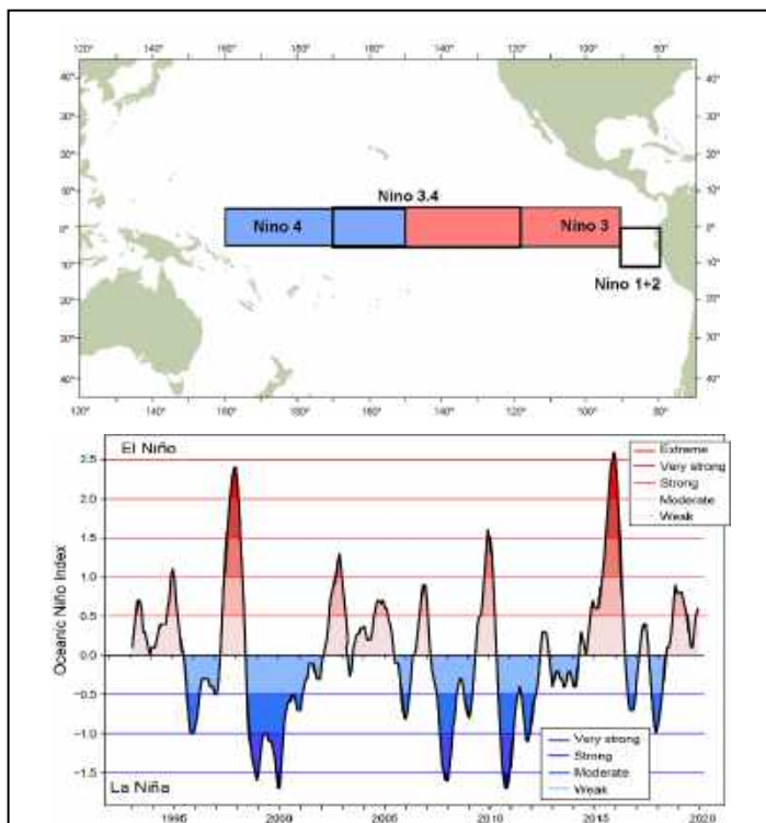
FIGURE L-7. El Niño regions used as indicators of El Niño Southern Oscillation (ENSO) events in the Pacific Ocean (top panel), and the Oceanic Niño Index (ONI) used to monitor ENSO conditions in Niño region 3.4 from 5°N to 5°S and 120°W to 170°W (bottom panel). Time series shows the running 3-month mean ONI values from the start of the IATTC observer program through December 2019. ONI data obtained from:
