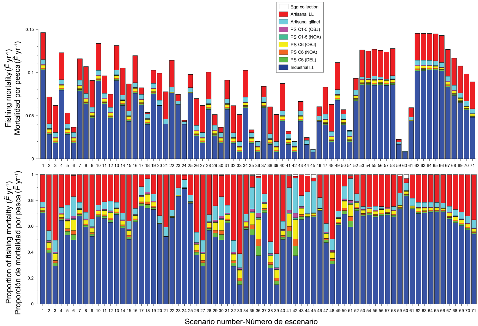
FIGURE 5. Mean values for the fishing mortality proxy ( \tilde{F}_{2019} ) for the East Pacific leatherback turtle ( Dermochelys coriacea ) stock estimated by EASI-Fish (top panel) and the proportion of total mortality \tilde{F}_{2019} value (bottom panel) for each conservation and management scenario based on the effort regime for industrial and artisanal fisheries in 2019 in the eastern Pacific Ocean. Descriptions of each scenario number show in the x-axis are provided in Table 5 and Table S1.
