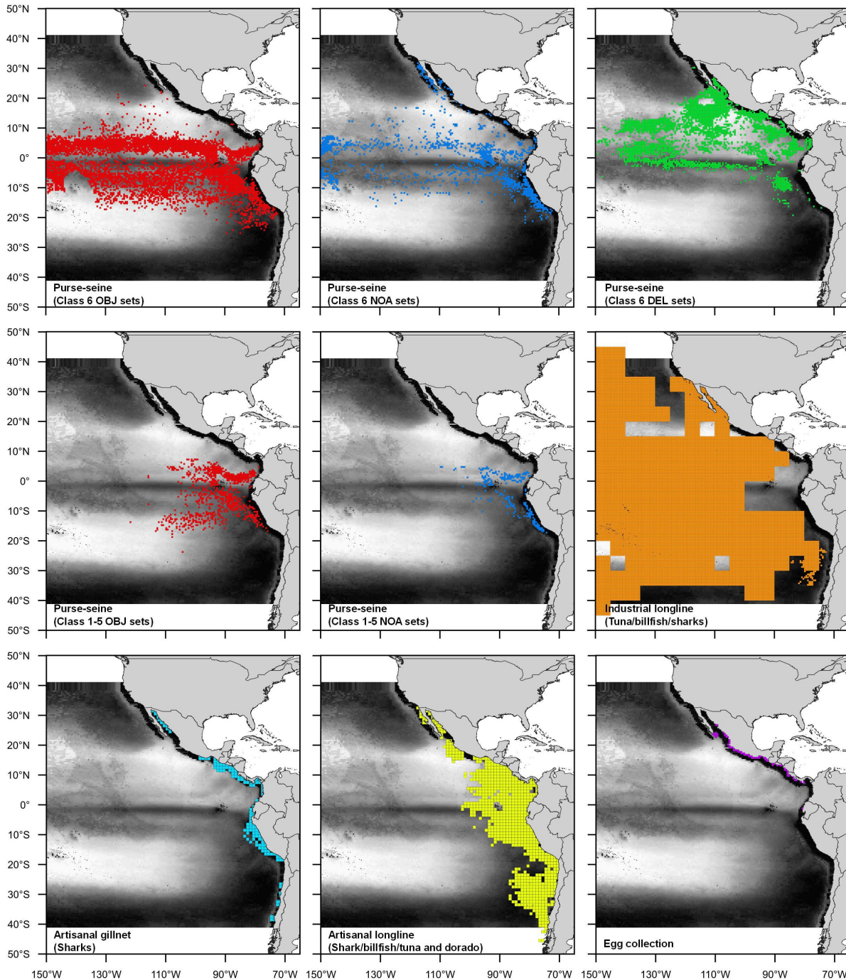
FIGURE 4. Maps showing the distribution of fishing effort by nine fisheries in the eastern Pacific Ocean in 2019 relative to the East Pacific stock of leatherback turtles ( Dermochelys coriacea ) (dark colors indicate higher probability of occurrence). Set types for the purse seine fisheries are: i) sets associated with floating objects (OBJ), ii) sets on unassociated schools of tuna (NOA), and iii) sets associated with dolphins (DEL).
