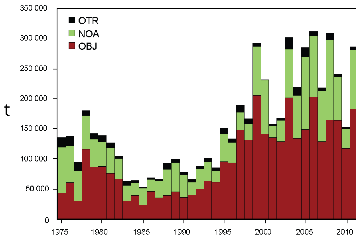
FIGURE C-1. Total catches (retained catches plus discards) of skipjack tuna by the purse-seine fisheries on floating objects and unassociated schools, and by other fisheries combined, in the eastern Pacific Ocean. The purse-seine catches are adjusted to the species composition estimate obtained from sampling the catches. The 2011 catch data are preliminary.
