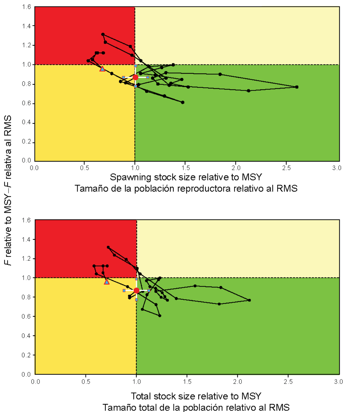
FIGURE B-6. Kobe (phase) plot of the time series of estimates for stock size (top: spawning biomass; bottom: summary biomass) and fishing mortality relative to their MSY reference points. Each dot is based on the average exploitation rate over three years; the large red dot indicates the most recent estimate. The squares around the most recent estimate represent its approximate 95% confidence interval.
