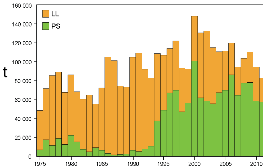
FIGURE D-3. Total catches (retained catches plus discards) of bigeye tuna by the purse-seine fisheries, and retained catches for the longline fisheries, in the eastern Pacific Ocean. The purse-seine catches are adjusted to the species composition estimate obtained from sampling the catches. The 2011 catch data are preliminary.
