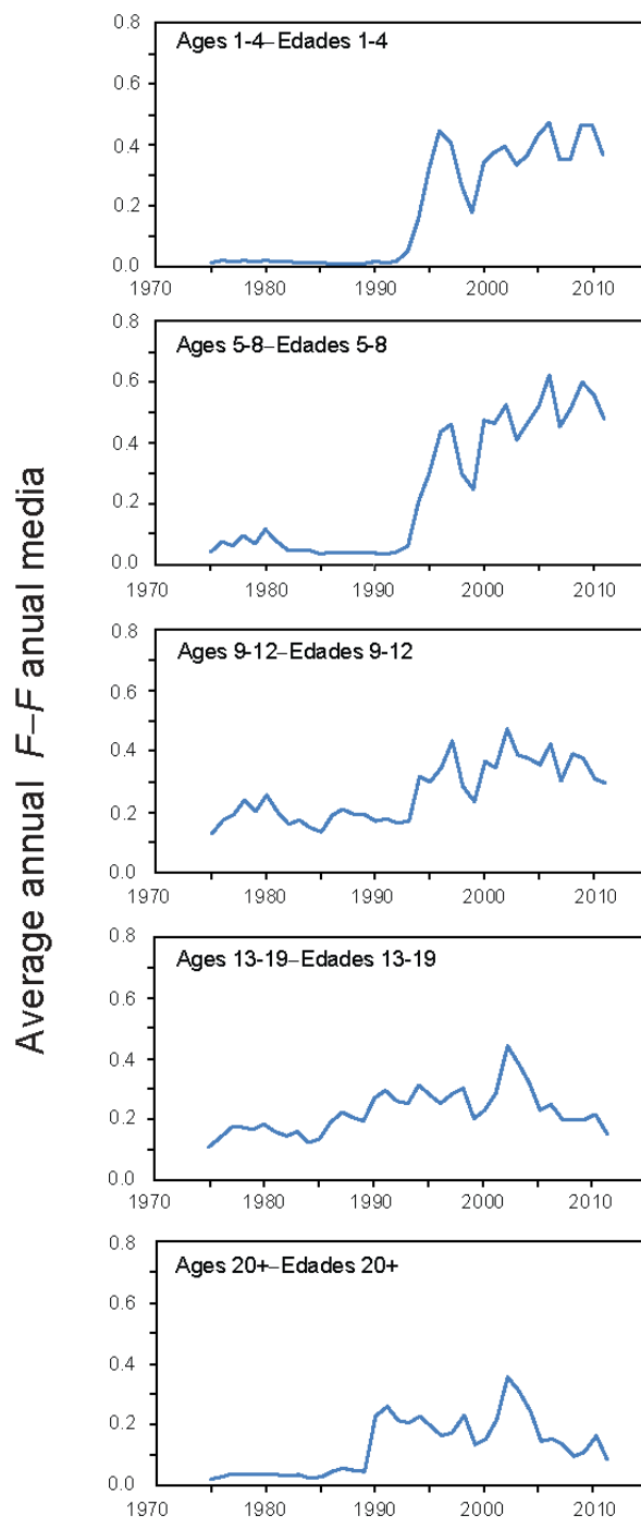
FIGURE D-4 Average annual fishing mortality, by all gears, of bigeye tuna recruited to the fisheries of the EPO. Each panel illustrates the average fishing mortality rates that affected the fish within the range of ages indicated in the title of each panel. For example, the trend illustrated in the top panel is an average of the fishing mortalities that affected the fish that were 1-4 quarters old.
