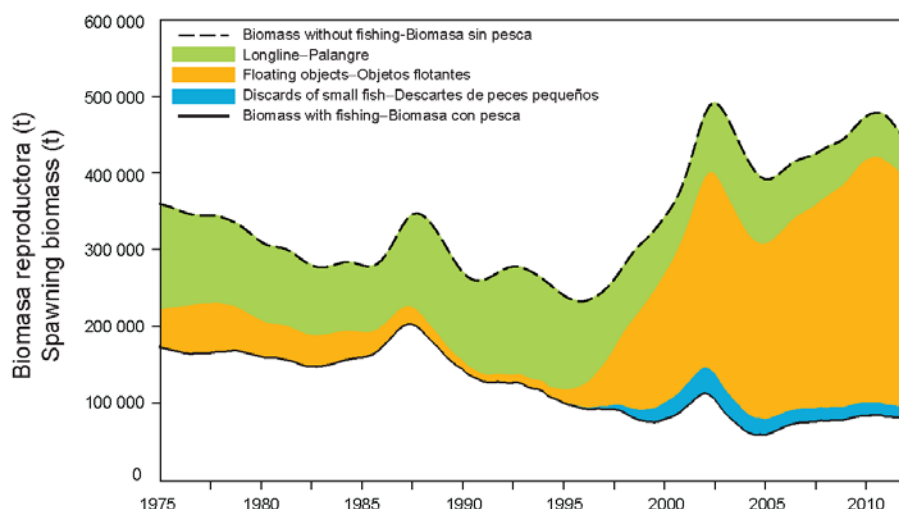
FIGURE D-5. Trajectory of the spawning biomass of a simulated population of bigeye tuna that was not exploited (top line) and that predicted by the stock assessment model (bottom line). The shaded areas between the two lines show the portions of the impact attributed to each fishing method. t = metric tons.
