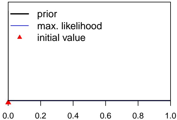
LnQ_base_EPO-LL-survey-early(24)
