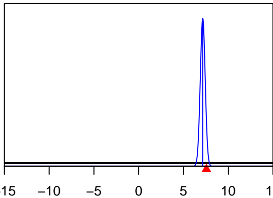
Size_DbIN_ascend_se_A2-LL-n(2)
