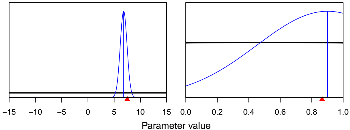
Size_DbIN_ascend_se_A6-OBJ(17)
