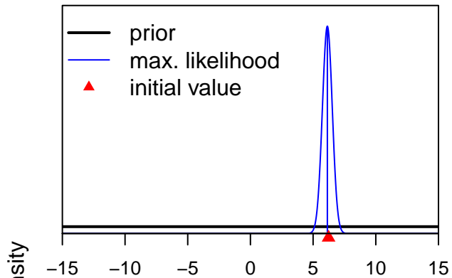
ize_DbIN_descend_se_A6-LL-n(6)_BLK2repl_1
