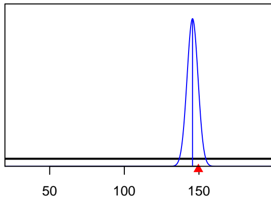
ize_DbIN_descend_se_A4-LL-n(4)_BLK2repl_1 Size_DbIN_top_logit_A5-LL-n(5)_BLK2repl_17
