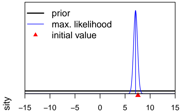
ize_DbIN_descend_se_A4-LL-n(4)_BLK2repl_1 Size_DbIN_top_logit_A5-LL-n(5)_BLK2repl_17
