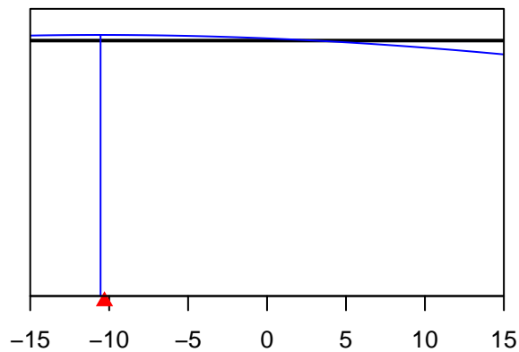
ize_DbIN_descend_se_A4-LL-n(4)_BLK2repl_1 Size_DbIN_top_logit_A5-LL-n(5)_BLK2repl_17
