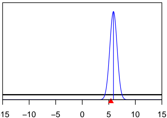
ize_DbIN_descend_se_A3-LL-n(3)_BLK2repl_1
