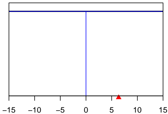
ize_DbIN_descend_se_A4-LL-n(4)_BLK2repl_1 Size_DbIN_top_logit_A5-LL-n(5)_BLK2repl_17
