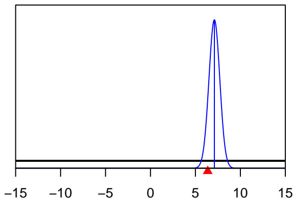
ize_DbIN_descend_se_EPO-LL-survey-late(25
