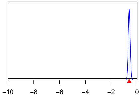
SizeSpline_GradHi_F11-NOA_N(11)
