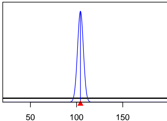
Size_DbIN_peak_F19-DEL_P(19)
