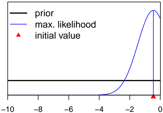
SizeSpline_Val_2_F9-OBJ_Cc_Q23(9)
