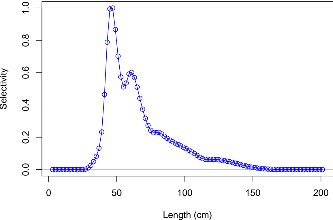
Female ending year selectivity for F1-Obj_N-Q14
