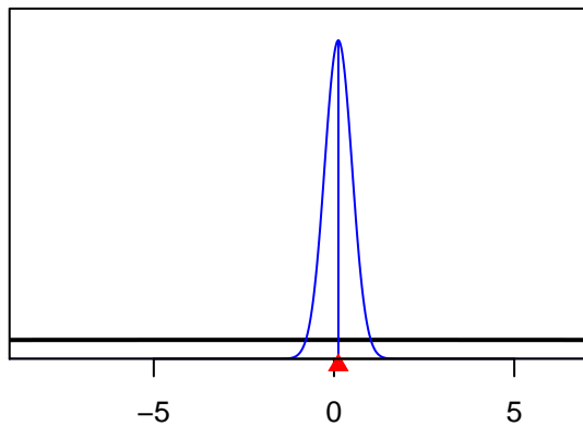
SizeSpline_Val_5_F7-OBJ_Nc_Q23(7)
