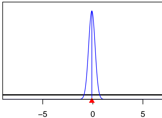
SizeSpline_Val_5_F7-OBJ_Nc_Q23(7)
