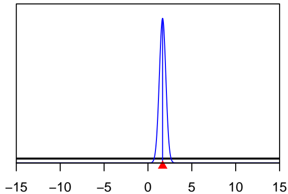
Q_power_S1-PS_DEL_VAST(41)
