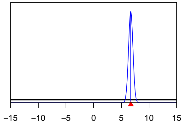
Size_DbIN_ascend_se_F19-DEL_P(19)
